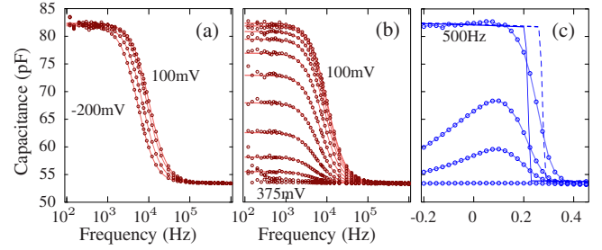
FIG. 5. (Color online) [(a) and (b)] Capacitance-frequency data from sample N taken over a sequence of V_{dc} for T=4.2 K and V_{ac}=5 mV rms . Points are data, lines are fits to data using the equivalent circuit of Fig. 2(b). According to our bias convention, n_S decreases with V_{dc} . (a) 100 mV steps in V_{dc} . The QW is occupied in all traces. (b) 25 mV steps in V_{dc} . This range of V_{dc} depletes the QW, reducing the low-frequency limit of the capacitance. (c) Capacitance-voltage data from the same device taken at various values of f (lines with symbols). Also shown are two charge-step simulations of the low-frequency capacitance with different QW \delta dopings: 1 \times 10^{11} cm -2 (solid line) and 2 \times 10^{11} cm -2 (dashed line). The abrupt step of the simulations is not observed in the data because the added impurities make the ground-state energy nonuniform across the sample.
