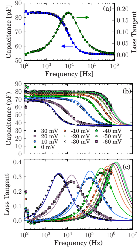
FIG. 11. (Color online) Measured capacitance and loss tangent versus frequency (symbols) and fits to both components of the data simultaneously using the equivalent circuit of Fig. 2(b) (lines). (a) Sample N measured at H=0 T, V_{dc}=0 V, and T=4.2 K. [(b) and (c)] Sample S measured at a variety of V_{dc} with T=5 K and H=6 T. The bias V_{dc}=30 mV corresponds to \nu=2 ; V_{dc}=-60 mV corresponds to midway between \nu=2 and 4.
